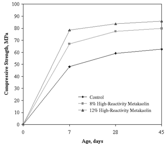
Fig. 1.4—Effect of high-reactivity metakaolin at 0.4 w/cm ratio on compressive strength of concrete (Hooton, Gruber, and Boddy 1997).
