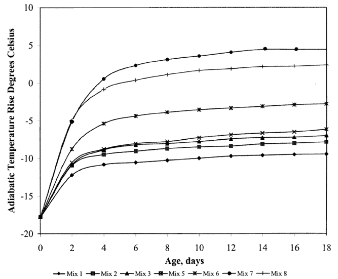
Fig. 2.16—Adiabatic temperature rise (1 kg/m 3 = 1.7 lb/yd 3 ) (Saad et al. 1982).
