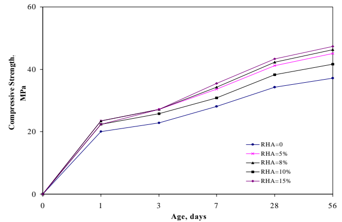
Fig. 2.3—Development of compressive strength of concrete with different percentages of RHA as cement replacement ( w/cm = 0.40 ) (Zhang and Malhotra 1996).
